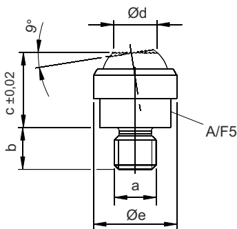
Design 5: swivel contact bolt, spherical, serrated contact face
