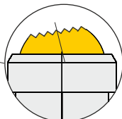
Design 5: swivel contact bolt, serrated contact face
